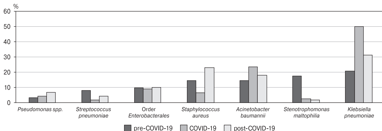
Figure. Structure of isolated microorganisms
